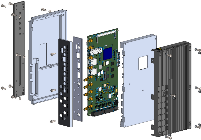
Figure 2 IFDR10 components
