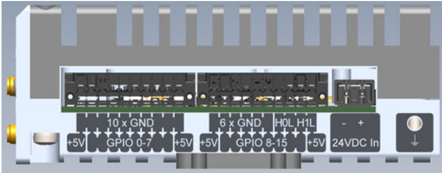
Figure 4 IFDR10 side connector panel
