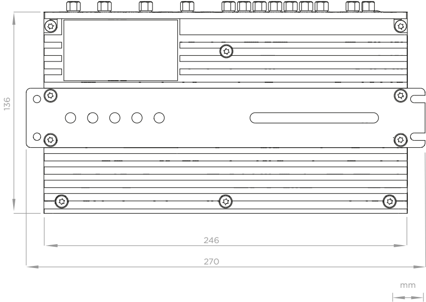
Figure 7 IFRD10 bottom view
