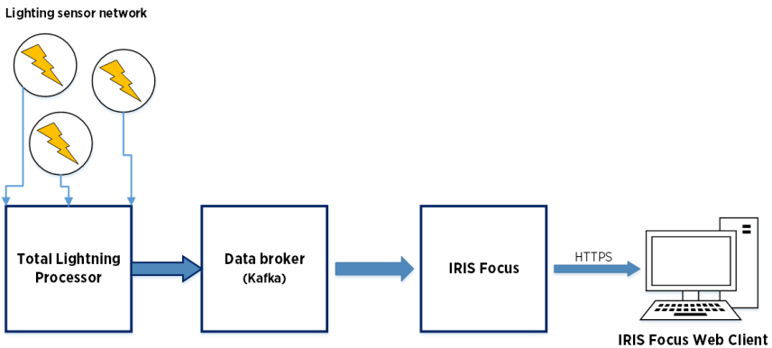
Figure 54 IRIS Focus lightning architecture
