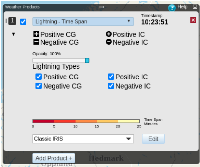
Figure 56 The TimeSpan product in the Weather Products pane
