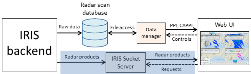
Figure 12 IRIS Analysis product data flow to IRIS Focus
