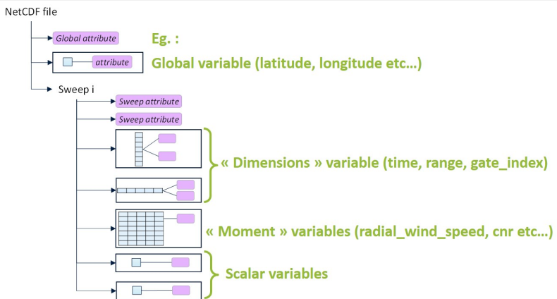
Figure 23 Vaisala NetCDF architecture
