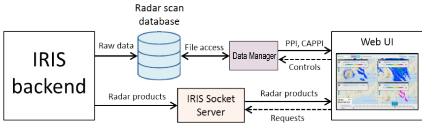
Figure 6 IRIS Focus architecture for radar products
