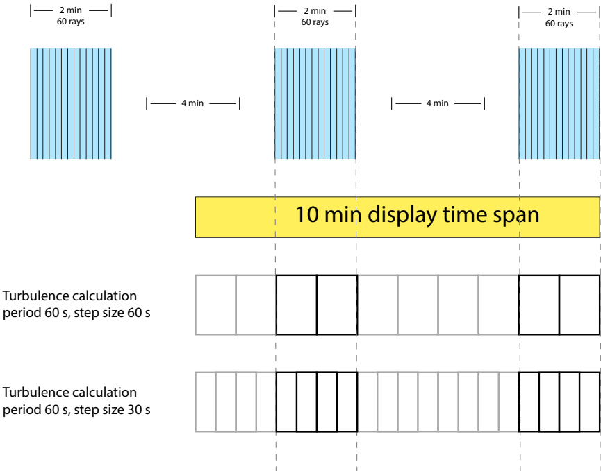
Figure 50 Turbulence calculation period and step size
