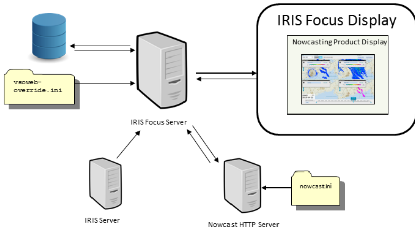
Figure 22 Nowcasting architecture
