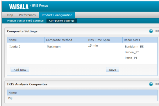
Figure 72 Composite settings
