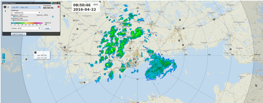
Figure 41 PPI example
