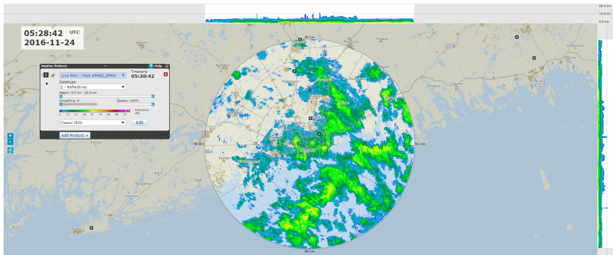
Figure 38 MAX example
