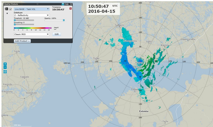
Figure 30 BASE example
