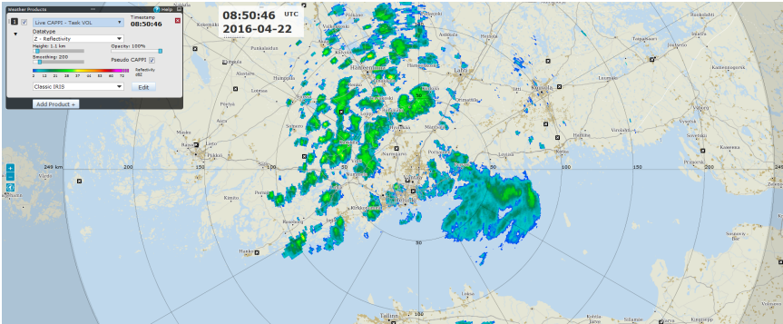
Figure 33 CAPPI example
