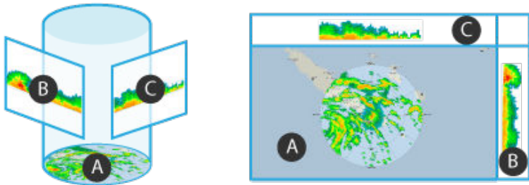
Figure 39 MAX views
