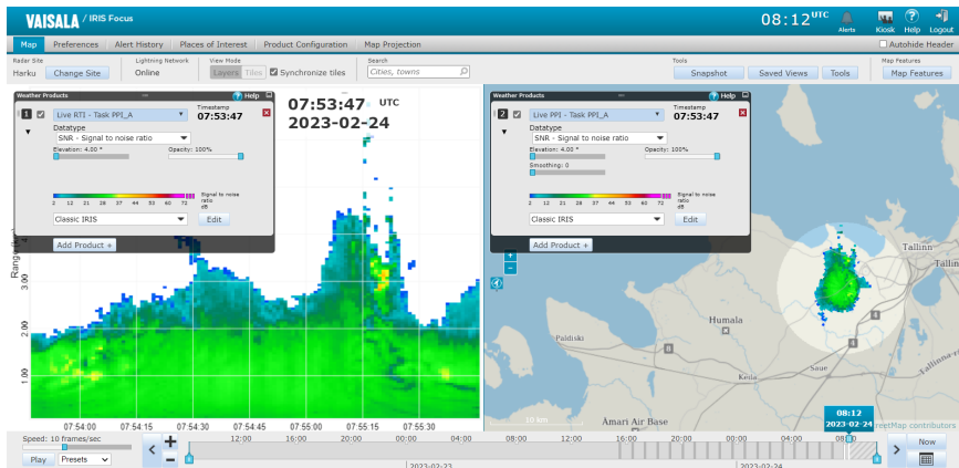
Figure 53 RTI example
