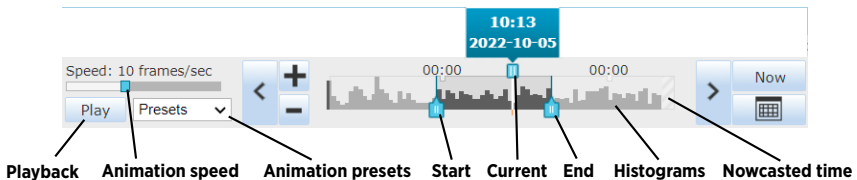
Figure 10 Animation controls
