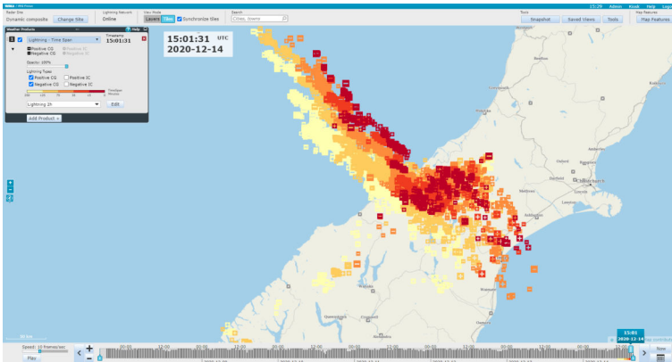
Figure 58 TimeSpan product
