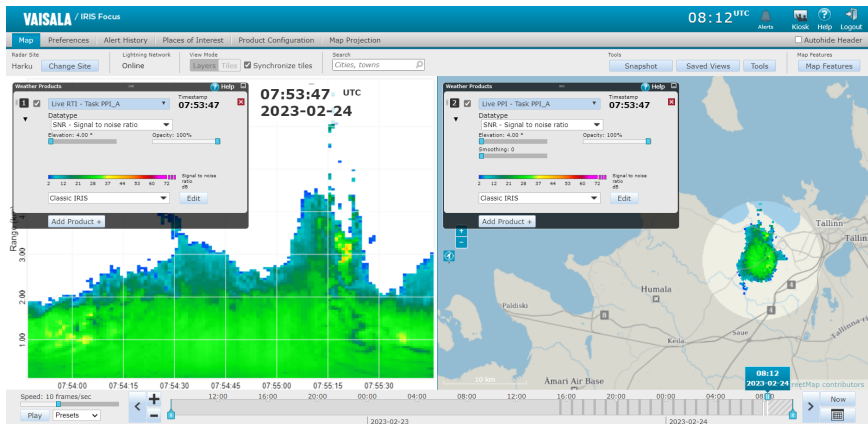
Figure 53 Exemple RTI
