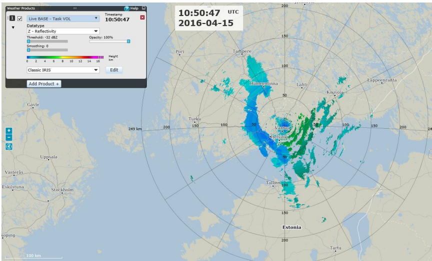
Figure 30 Exemple BASE
